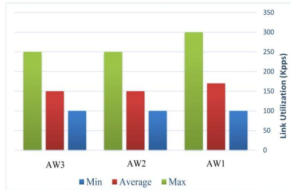
Figure 4- Link Utilization for Sample AW1 to AW3
