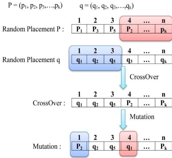
Figure 3-state chart of Genetic algorithm
