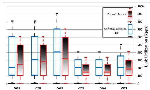
Figure 6-comparison of the link utilization
