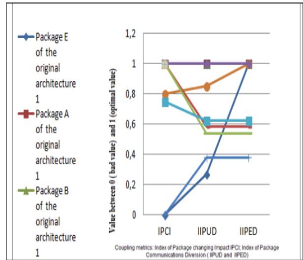
Fig. 7 Graphic representation of Coupling metrics: Index of Package changing Impact; Index of Package Communications Diversion (table3).
