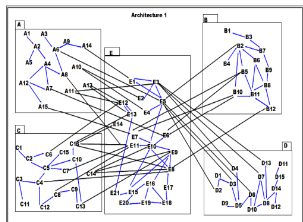
Fig. 1 An initial architecture composed of classes and packages
