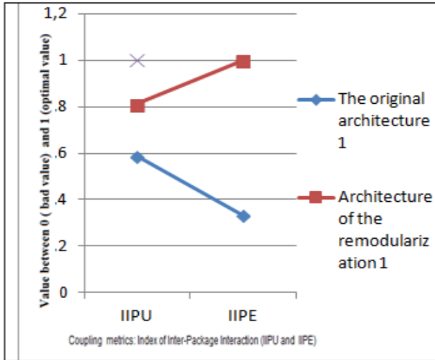
Fig. 6 Graphic representation of Coupling metrics: Index of Inter-Package IIPU and IPE (table2).
