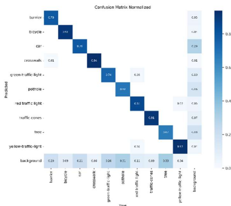
Fig. 5. Confusion matrix for Yolov8 (crossing road)
