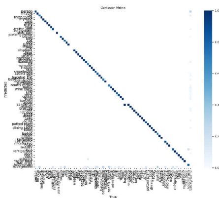
Fig. 6. Confusion matrix for Yolov5 (Search for object)
