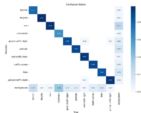
Fig. 4. Confusion matrix for Yolov(crossing road)
