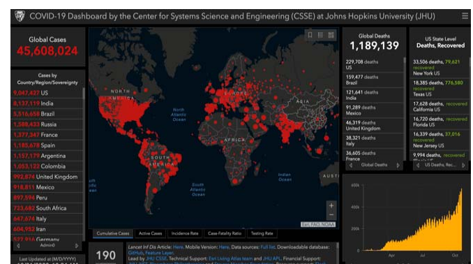
Fig .1 Total Case, Total Death from (JHU).
