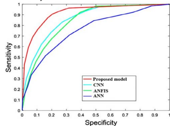
Figure 4: ROC obtained
