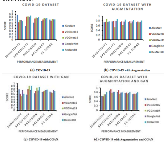
Figure 9: Performance metrics of CT datasets
